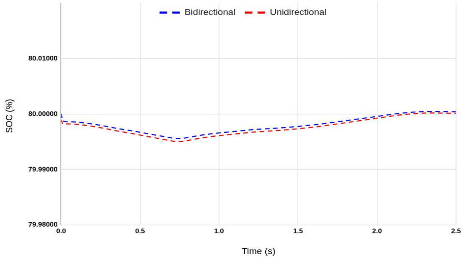
Fig. 3 The battery state-of-charge for both converters
